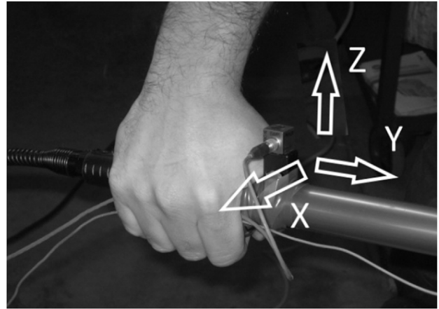
Fig. 3. A triaxial accelerometer positioned near the hand.
