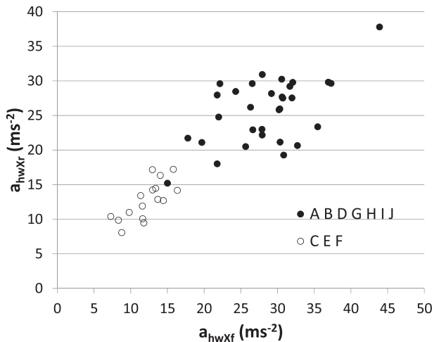
Fig. 7. Graphical illustration of the two clusters found by cluster analysis.
