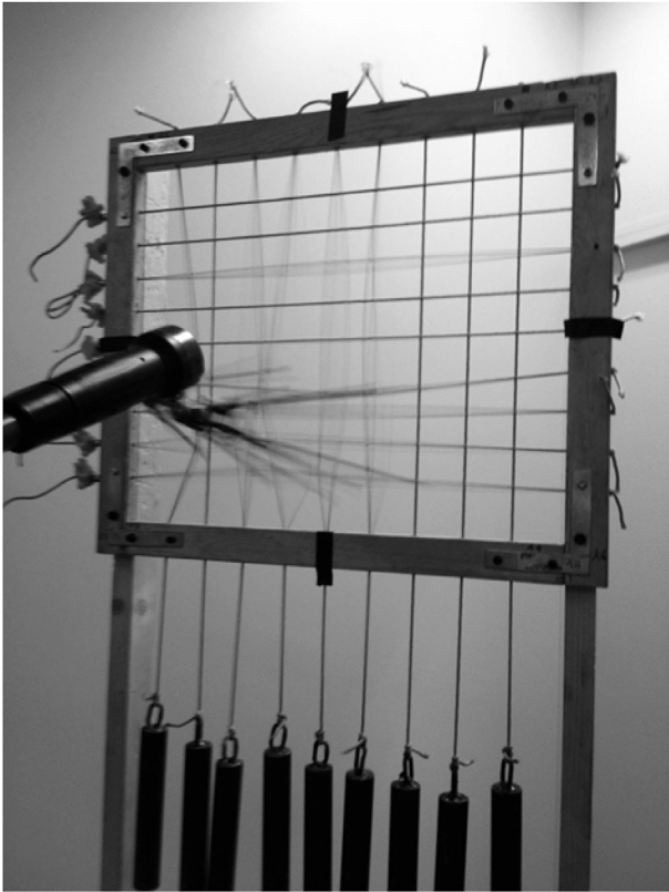
Fig. 2. The harvester interacting with the tree simulator.
