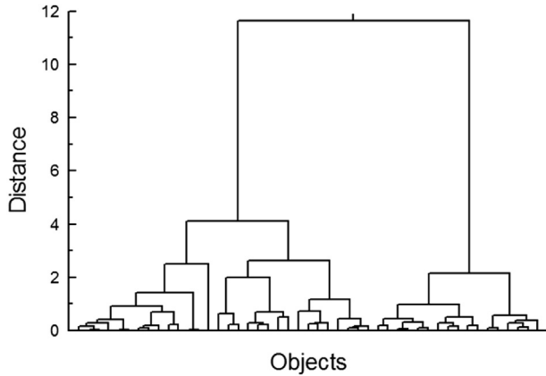
Fig. 6. Dendrogram of hierarchical clustering.
