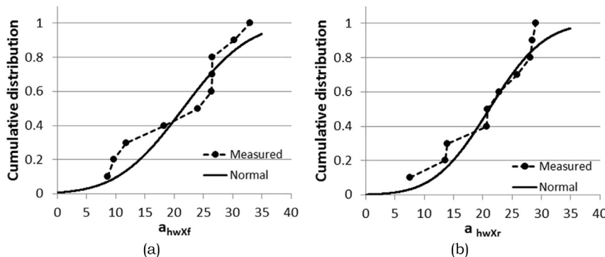
Fig. 5. Experimental (dashed line) and normal (solid line) distributions of the front (a) and rear (b) X-axis accelerations in the ten laboratories.
