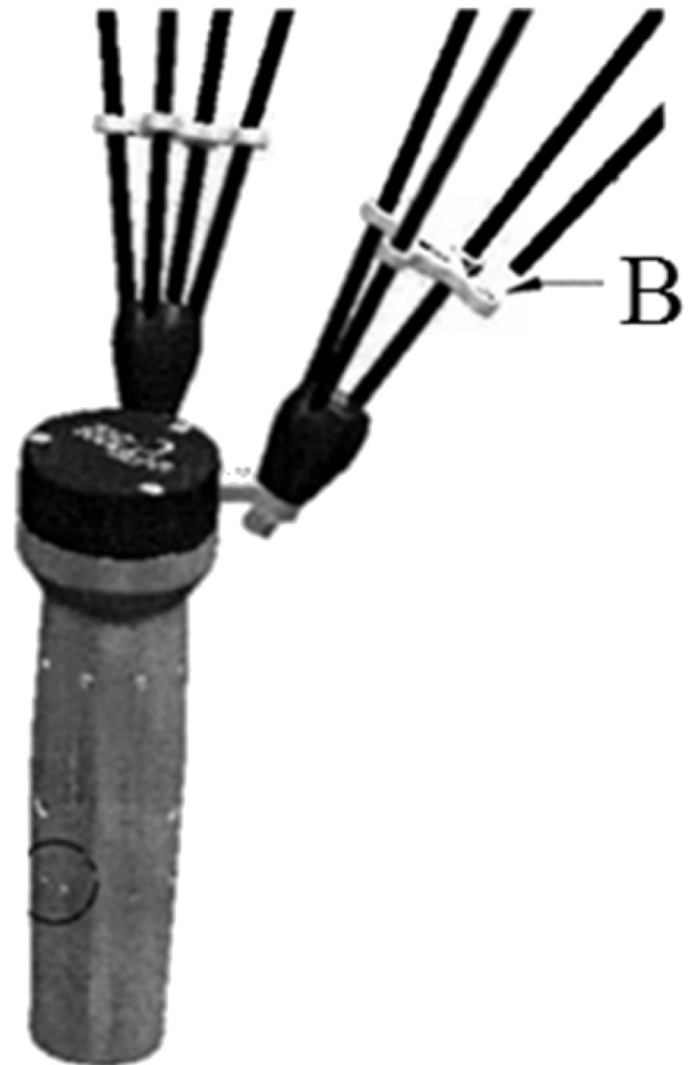
Fig. 8. Graphical instructions for the mounting of the anti-breaking devices (extracted from the beater user manual).
